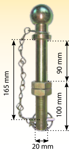
Ball Pin & Chain 7 1/2" x 1"
