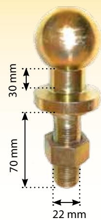
Short Ball Hitch Pin 7/8"
