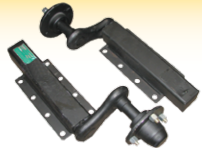
Trailer 750kg Suspension Unit Per Pair 4" PCD Hubs 4 Stud Grease Nipples
