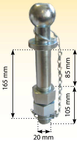
Hitch Pin and Ball 1 1/4"
