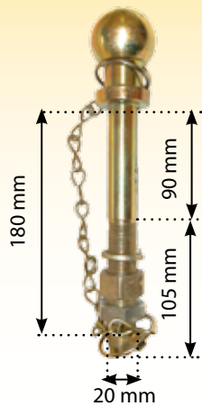
Ball Pin & Chain 7 1/2" x 7/8"
