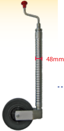
Trailer Jockey Wheel Barrel Diameter 48mm
